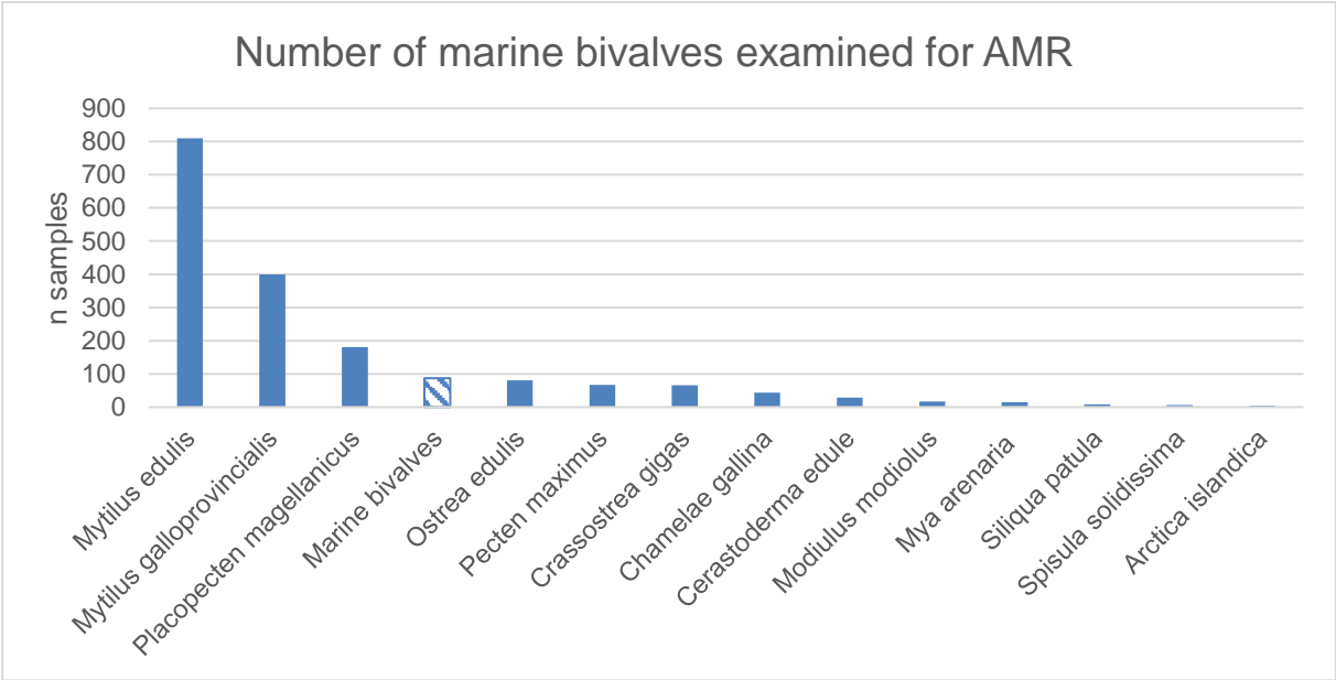
Figure 2: Overview of the number of examined marine bivalve samples, by species. The bar “Marine bivalves” include samples where the species is not specified.
