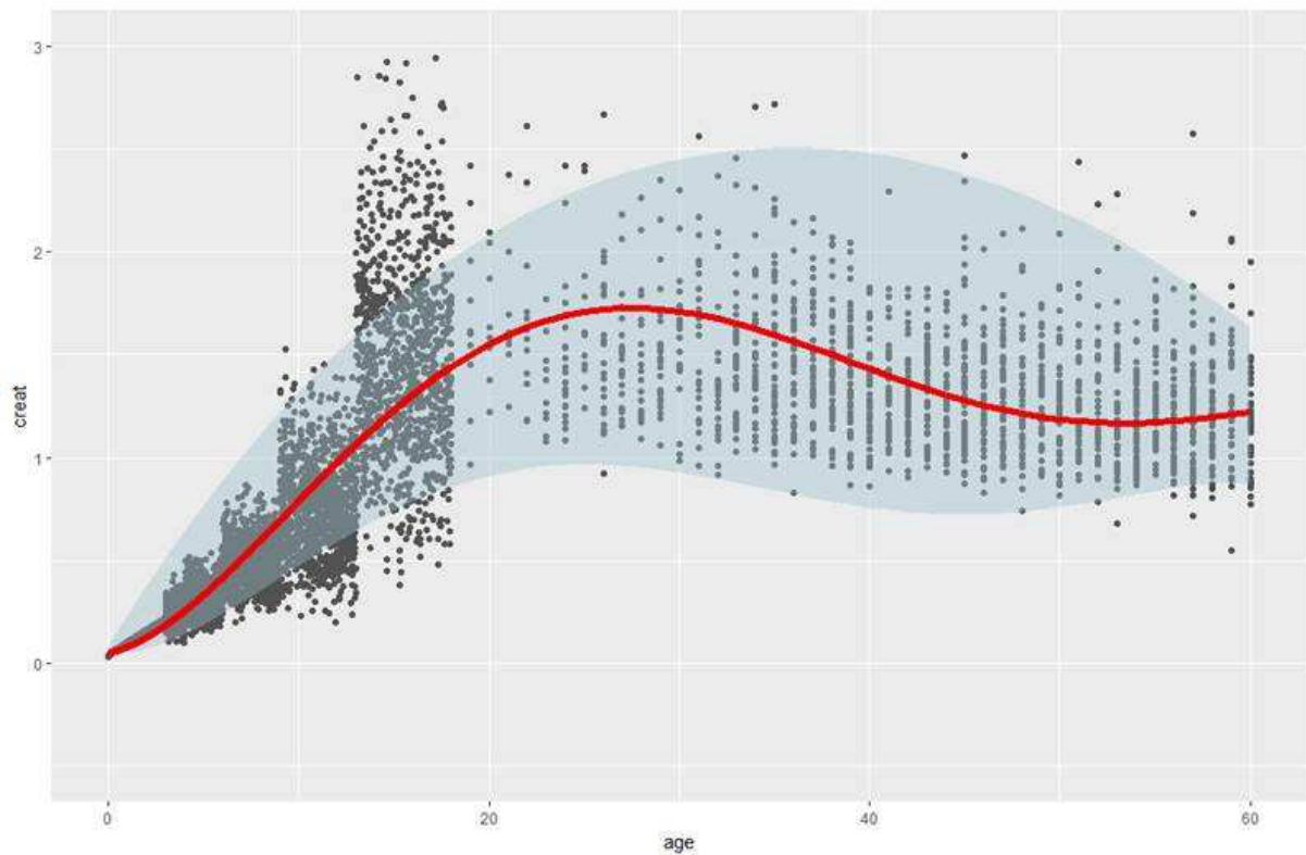
271 Figure 1: Change in creatinine excretion with age based on the observed data from French 272 Nutrition and Health Survey (ENNS, Castetbon et al., 2009) for adults (>18 years) and data from 273 Remer et al. (Remer et al.,2012) for children.
