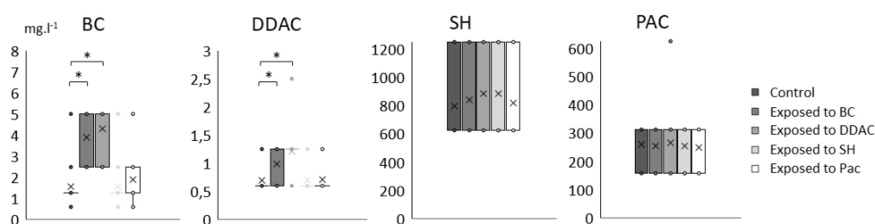
Figure 2. Variation of MIC values ( \text{mg}\cdot\text{L}^{-1} ) of benzalkonium chloride (BC), dimethylammonium chloride (DDAC), sodium hypochlorite (SH) and peracetic acid (PAC) for the 28 selected Lm strains exposed or not (control) to the 4 biocides. Significant difference with control is indicated by star (*, paired T-test, p -value < 0.01 ). Boxes range from the 25th to 75th percentile and whiskers extending below and above the box range from the lowest to the upper value, respectively. Cross (×) indicates the median, circles (○) correspond to outlier values.
