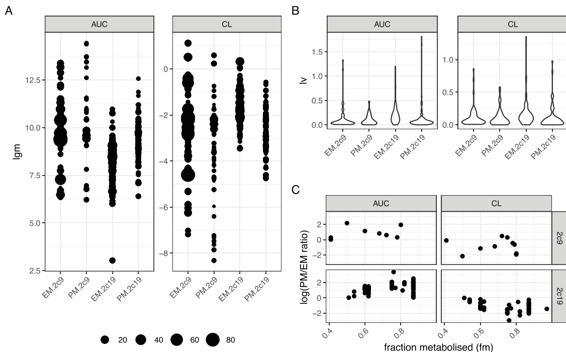
Fig. 2. Distribution of input data (A. logarithms of sample geometric means, lgm; B. logarithms of sample variations, lv; C. ratios of geometric means between poor metabolisers PMs and extensive metabolisers EMs, according to Fm).
