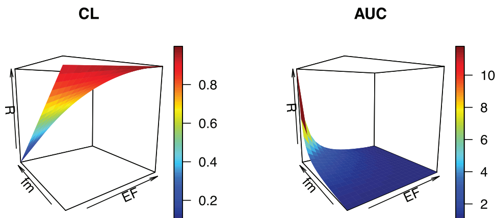
Fig. 1. Relationship between fraction metabolised Fm, enzyme function EF and geometric mean ratio R.
