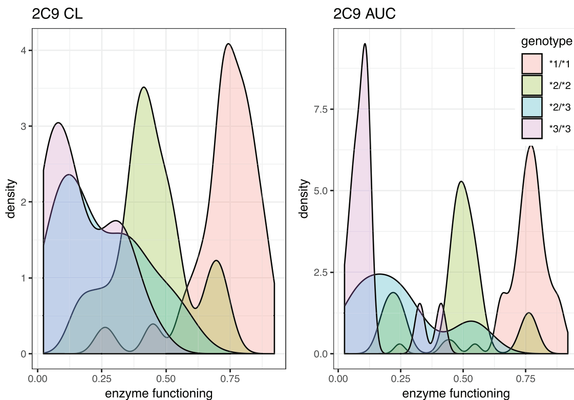
Fig. 3. Distributions of mean EFs in human subpopulations for CYP2C9 clearance and AUC parameters.
