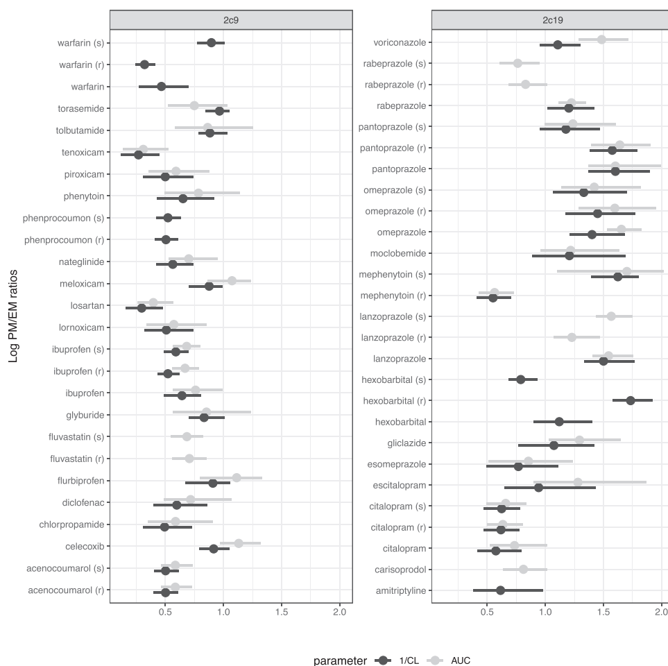
Fig. 4. Inter-phenotypic differences in the pharmacokinetics of CYP2C9 and CYP2C19 probe substrates for markers of chronic exposure (clearance, CL and AUC) expressed as ratios of geometric means, on log scale, between poor metabolisers PMs and extensive metabolisers EMs. To allow for comparison across CL and AUC, reciprocal of CL was used.
