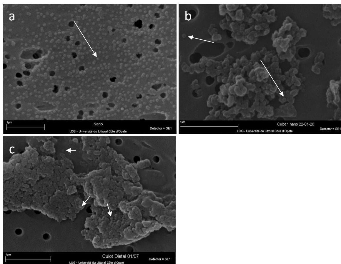
Fig. 4 : Observation of nanoplastics by scanning electron microscopy. (a) Sample of aqueous suspension of polystyrene nanoplastic beads (PS-NP) at the concentration of 5000 \text{ mg L}^{-1} in Krebs-Glucose (latex beads amine-modified polystyrene 0.05 \text{ } \mu\text{m} mean particle size, Sigma-Aldrich, France); (b) sample of the same aqueous PS-NP dispersion after the TCA precipitation protocol (see details in material and methods section); (c) sample of Krebs-Glucose solution collected from the serous side of the distal portion of the intestine, at the end of the 150-min kinetic experiment during which the PS-NP dispersion diluted at 200 \text{ mg L}^{-1} was added to the luminal side at T0, and washed according to the TCA precipitation protocol. The white arrows show the nanoplastic beads observed.
