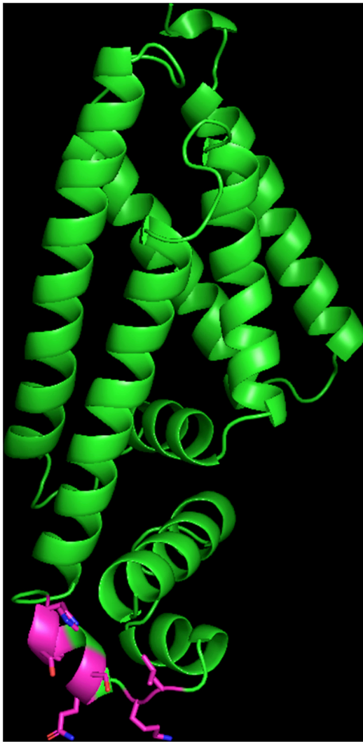
FIGURE 1 | Structure of the FepR protein. The carbon of the side chain of the mutated residues inside the HTH domain are shown in pink. Oxygen atoms are shown in red and nitrogen in blue. Hydrogen atoms are hidden.
