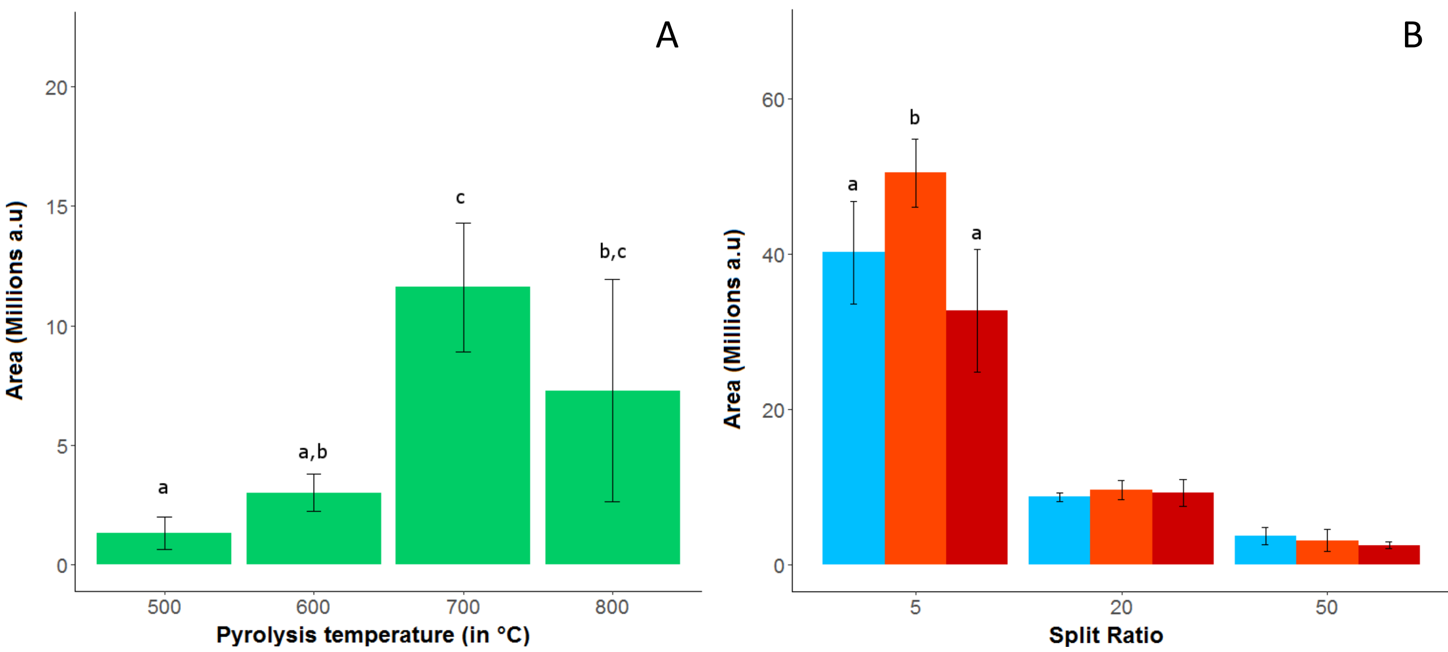
Figure 3: Mean peak area (arbitrary unit) depending on the Pyrolysis temperature (A), on split ratio and injector temperature (blue: 280 °C, orange: 300 °C and red: 320 °C) (B) of the 1-decene (PE). Error bars correspond to the CI95% and letters to the differences after post-hoc using Fisher's least significant difference with Bonferroni correction.
