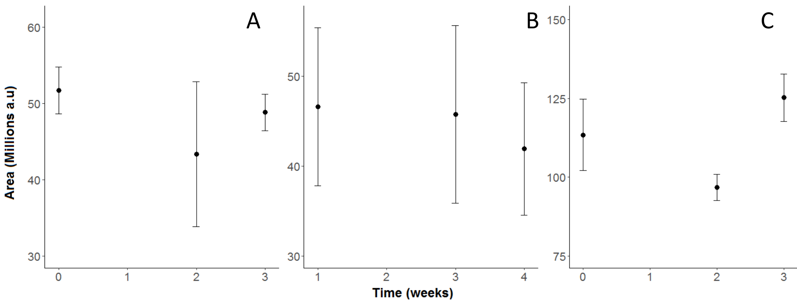
Figure 4: Mean peak area (arbitrary unit) over time (in weeks) for the mains peaks of PE (A), PS (B) and PMMA (C). Errors bars correspond to the CI95%.
