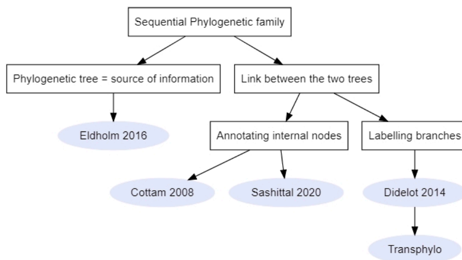
Figure 5. Links between methods of the sequential phylogenetic family. Rectangles represent criteria on which to choose a method and the grey circles represent either the name of the method's package or the first author and article date [2,17,31,39].
