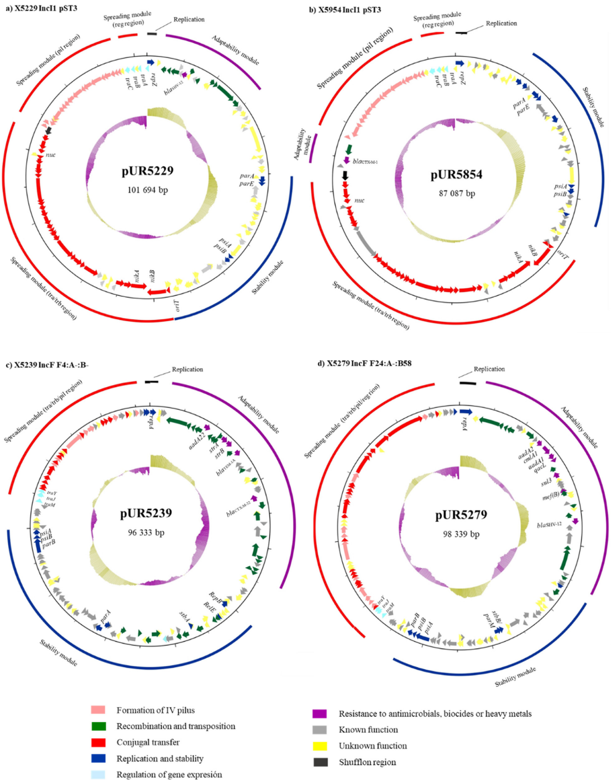
Fig. 2. Circular map of the four bla ESBL -carrying plasmids (A) pUR5229 (accession number Q0658192 ), (B) pUR5854 (accession number Q0747076 ), (C) pUR5239 (accession number Q0747074 ), and (D) pUR5279 (accession number Q0747075 ).
