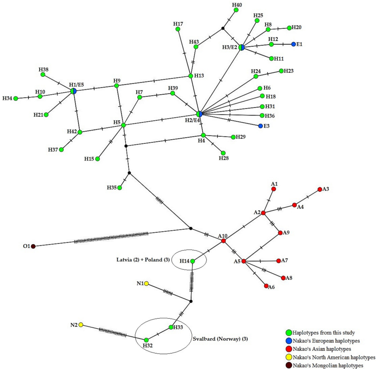
Fig. 3. Haplotype network sensu Nakao. TCS network representing the relationship between the 36 Echinococcus multilocularis cob + nad2 + cox1 haplotypes (3,558 bp) detected in this study (in green) and the Nakao historical haplotypes, designated as European, Asian, North American and Mongolian. In this network, former H16, H19, H22 and H27 are incorporated in H2, H41 is incorporated in H3, H30 is incorporated in H4 and H26 are incorporated in H24. Each haplotype is represented by a circle, with the area of the circle proportional to its frequency. Hatch marks depict single mutational steps and small dots display hypothetical haplotypes. A colour version of this figure is available on-line.
