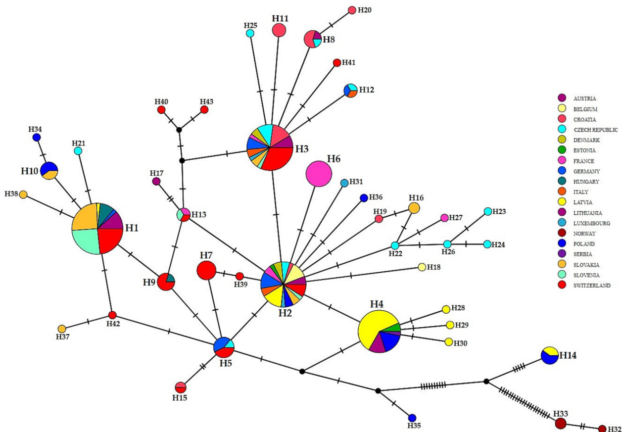
Fig. 1. Haplotype network. TCS network representing the 43 Echinococcus multilocularis cox1 haplotypes (4,968 bp) detected in this study, obtained from 227 isolates. Each haplotype is represented by a circle, with the area of the circle proportional to its frequency. Hatches depict single mutational steps and small black dots display hypothetical haplotypes. A colour version of this figure is available on-line.
