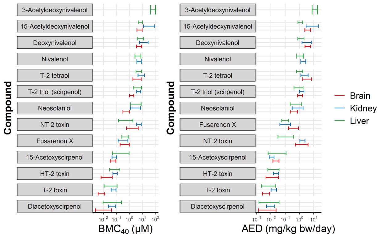
Fig. 3. Potency ranking of trichothecenes based on benchmark concentration modeling (left; units in μM; IVIVE not applied) and benchmark concentration modeling coupled with in vitro-in vivo extrapolation (right; units in mg/kg bw/day).
