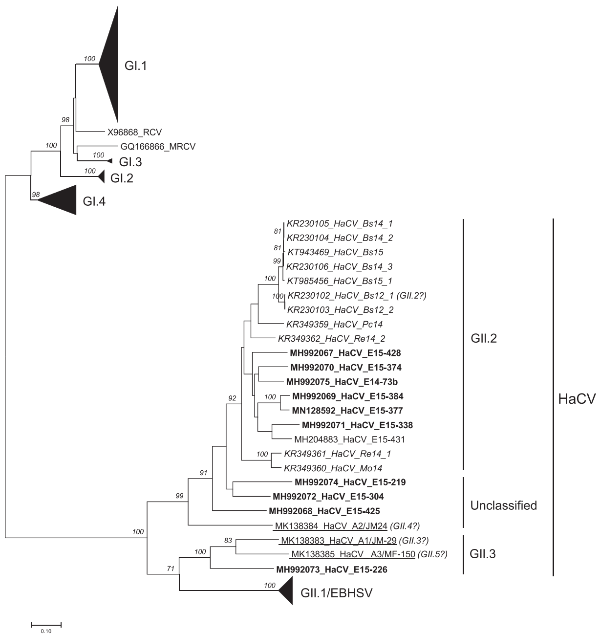
Fig. 1. Maximum likelihood phylogenetic tree of complete and nearly complete lagovirus VP60 gene nucleotide sequences ( n = 190 ). The maximum likelihood method (MEGA software version 7; Kumar et al., 2016) was implemented with the GTR + \Gamma model of nucleotide substitution and a NNI branch-swapping. The Jalview2 software (Waterhouse et al., 2009) was used to reduce the number of available sequences in nucleotide databases (redundancy threshold of 98). The final dataset is 190 sequences. The tree was rooted using GI viruses. Significant bootstrap values greater than 70 for 1000 replicates are shown in italic after each node. Lagovirus genotypes GI.1–4 and GII.1 are represented as collapsed in order to reduce the tree size and highlight the HaCV sequences. French HaCV sequenced in this study are shown in bold, Italian HaCV in italics and Australian HaCV are underlined. The four putative HaCV genotypes (GII.2–4?) previously suggested by Le Pendu et al. (2017) and Mahar et al. (2019) are indicated in italics for the corresponding HaCV strains.
