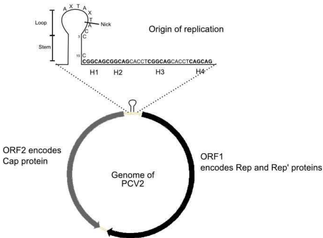
Figure 1 Representation of genome of PCV-2. Black arrow: Open Reading Frame 1 (ORF1), located on the positive strand, which encodes Rep and Rep' protein. Grey arrow: Open Reading Frame 2 (ORF2), located on the negative strand, which encodes Cap protein. Between ORF1 and ORF2 are intergenic regions. The origin of replication is located in the intergenic region between the beginnings of the two ORFs. H1, H2, H3 and H4 are hexamers.
